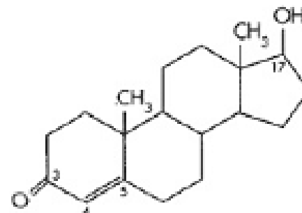
Testosterona
